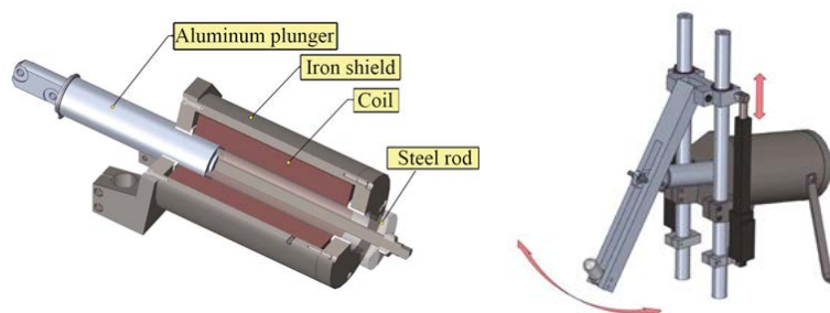
Fig. 4. The electromagnet shooting system of the NuBot soccer robot. Left: The Electromagnet; right: The Shooting System.
